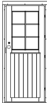
Single Door tempered gl 1 st. 70 mm 840 x 1955 mm
